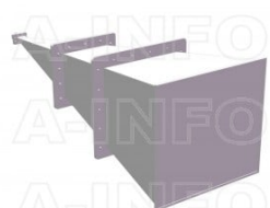
LB-137-25-C-SFSPO Standard Gain Horn Antenna 5.85-8.2GHz 25dB Gain SMA Female
