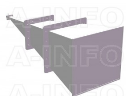
LB-137-25-C-TFSPO Standard Gain Horn Antenna 5.85-8.2GHz 25dB Gain TNC Female
