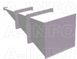
LB-137-25-C-NFSPO Standard Gain Horn Antenna 5.85-8.2GHz 25dB Gain N Type Female
